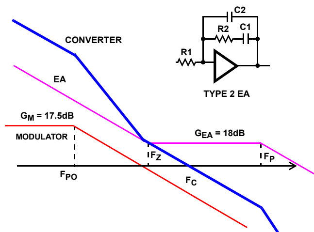
FIGURE 19. FEEDBACK LOOP COMPENSATION
