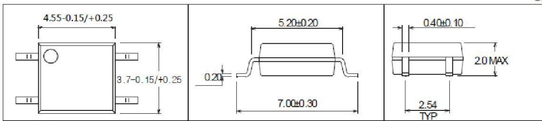
4-pin SOP
