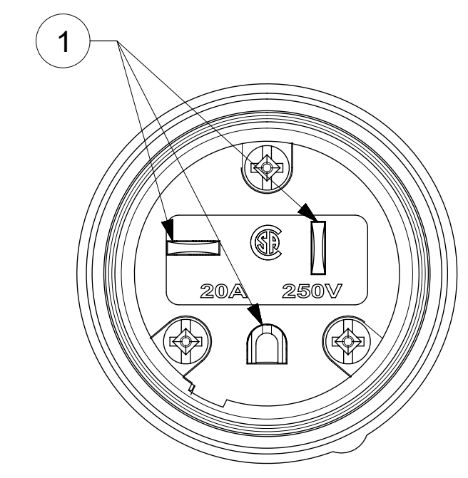
FACE VIEW
