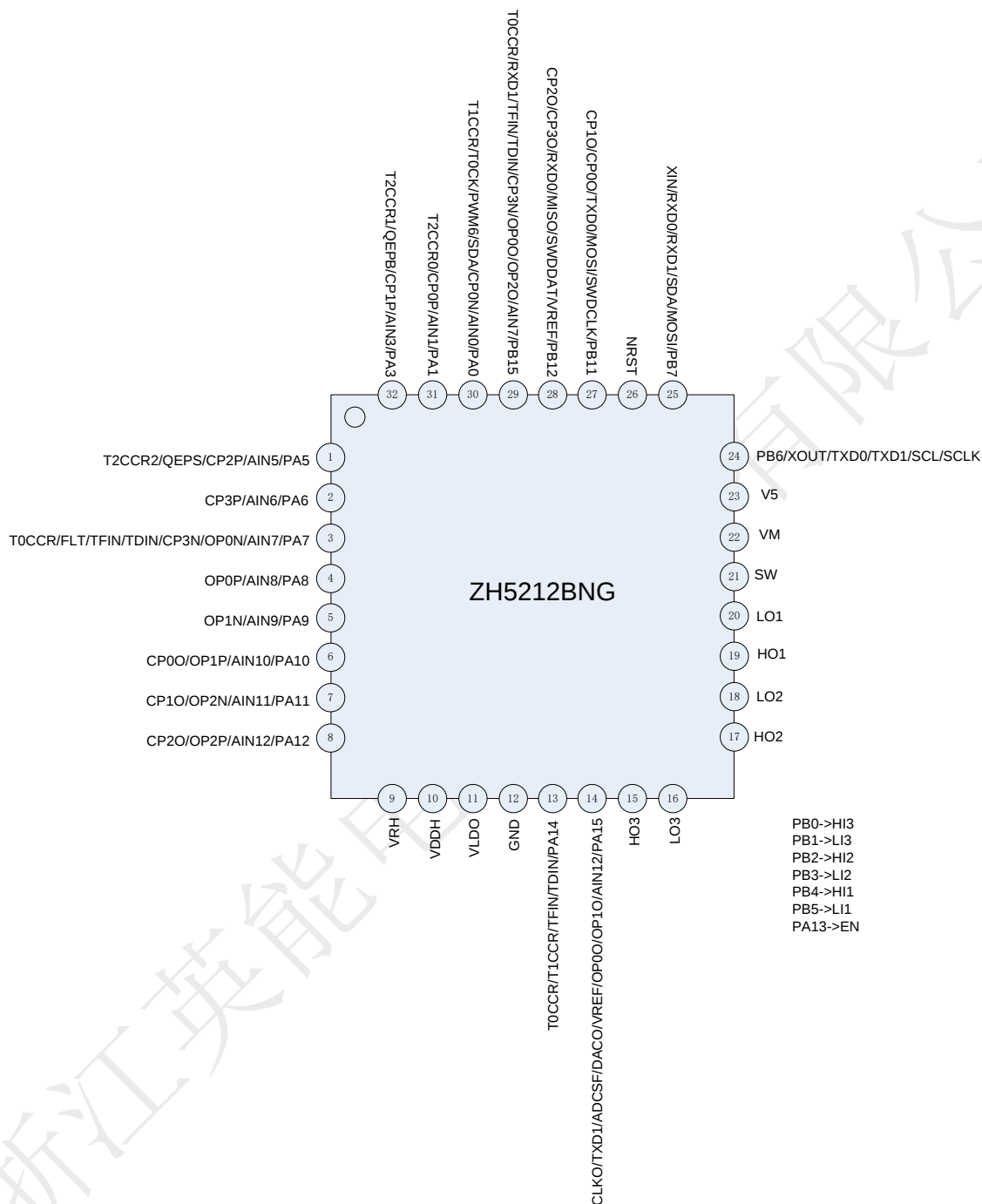
图 3-1-7 ZH5212BNG(QFN32)引脚图
