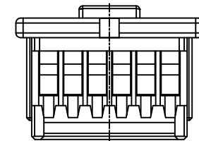
X1004H-XXA-N0HF 06-15Pin
