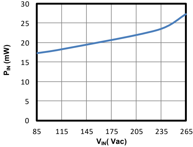
No-Load Consumption
