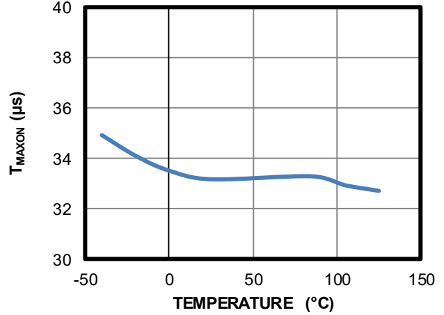
Open-Loop Detection vs. Temperature
