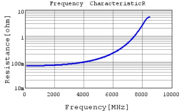
GQM2195G2E2R7BB12 R DC0V, 25degC
