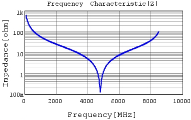
GQM2195G2E2R7BB12 |Z| DC0V, 25degC
