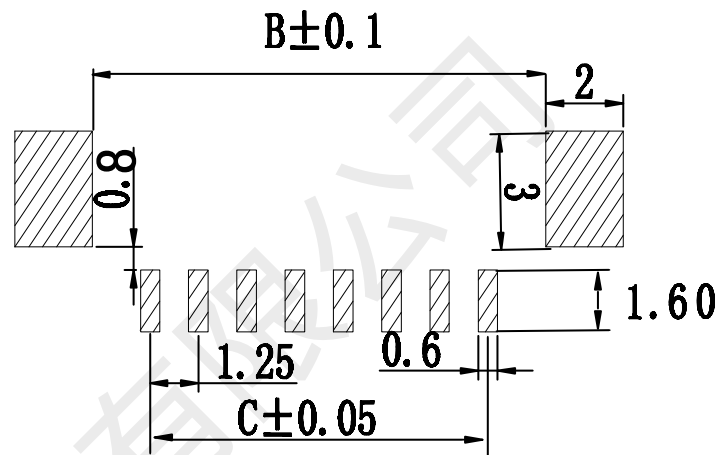
RECOMMENDED P. C. BOARD LAYOUT (TOP VIEW)
