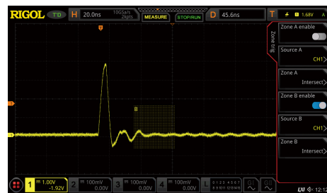
Quickly isolate the exceptional signal with Edge trigger and Zone trigger.
