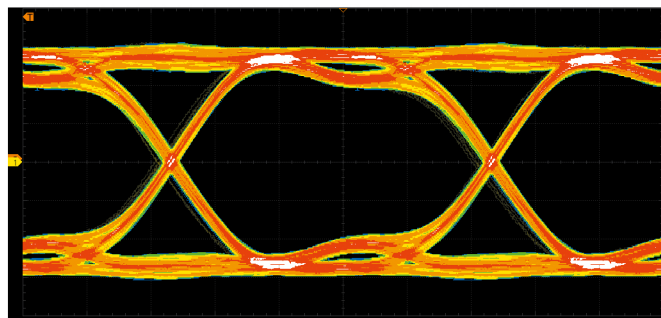
Use the 600 MHz bandwidth and 1 GHz bandwidth model respectively to perform eye measurement on the 1 Gb/s signal.
