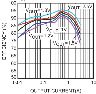
Efficiency vs. Output Voltage V_{IN} = 3.3V
