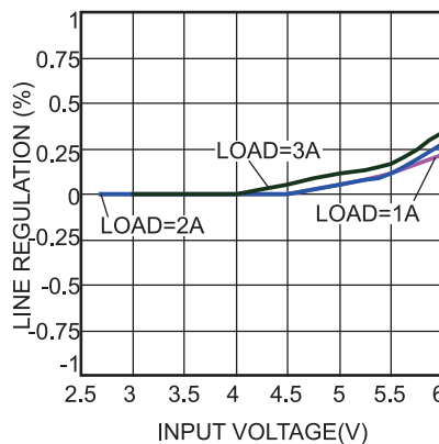
Line Regulation
