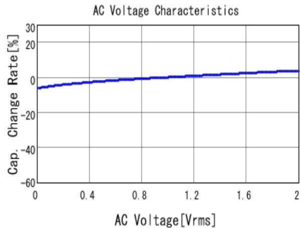
■ GRM15XR61A223KA86 C-AC Voltage capchange, DC0V, 25.0d
