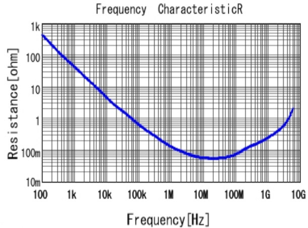
■ GRM15XR61A223KA86 R DC0V, 25degC
