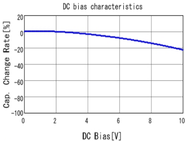
■ GRM15XR61A223KA86 C-DC bias capchange, 25.0degC, AC1.
