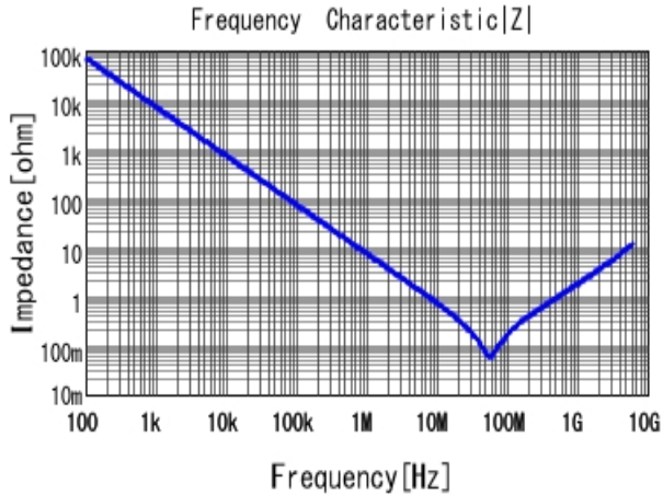
■ GRM15XR61A223KA86 |Z| DC0V, 25degC
