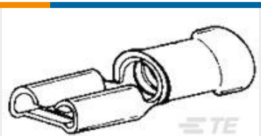
TE Part #140805-2 TERMINAL REC FASTON PIDG 5
