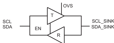
Figure 33. I²C Drivers in TMDS442
