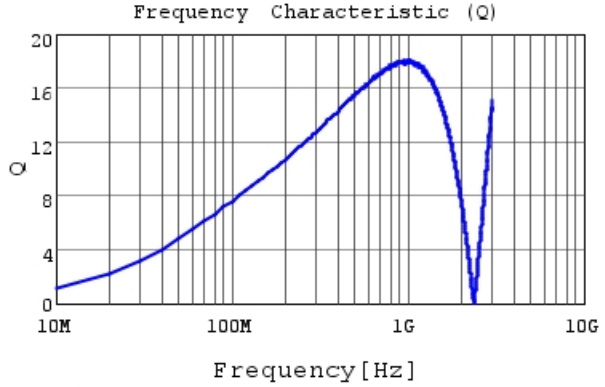
LQP03TN39NJ02 Q
