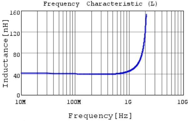
LQP03TN39NJ02 L
