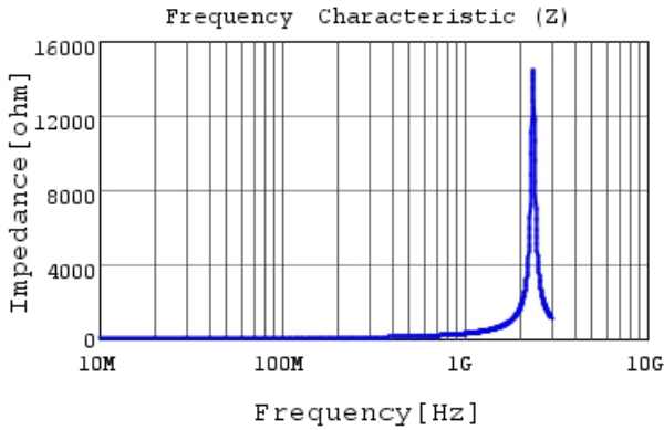
LQP03TN39NJ02 |Z|
