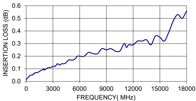
141-6SM+ INSERTION LOSS
