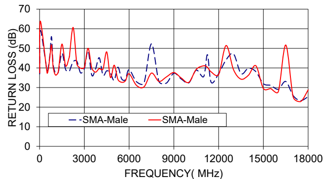
141-6SM+ RETURN LOSS
