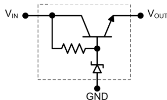
Internal Device Schematic
