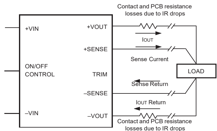
Figure 4. Remote Sense Circuit Configuration
