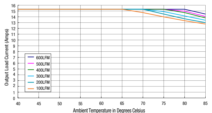
Maximum Current Temperature Derating at Sea Level ( V_{in} = 75V , airflow is from V_{in-} to V_{in+} )
