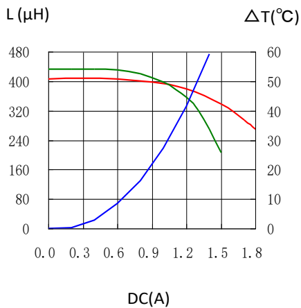
CDRH127/HPNP-391MC
