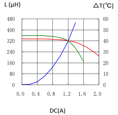
CDRH127/HPNP-331MC
