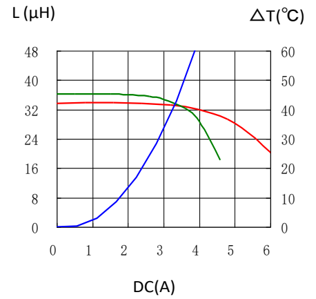
CDRH127/HPNP-330MC
