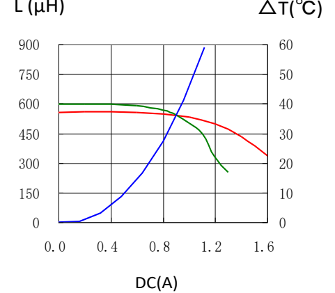
CDRH127/HPNP-561MC
