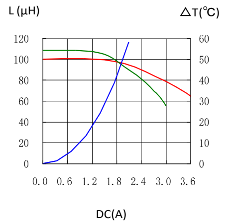
CDRH127/HPNP-101MC
