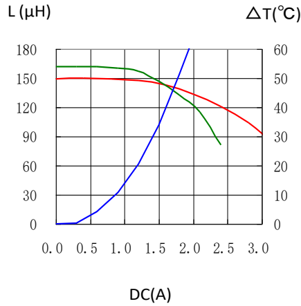
CDRH127/HPNP-151MC
