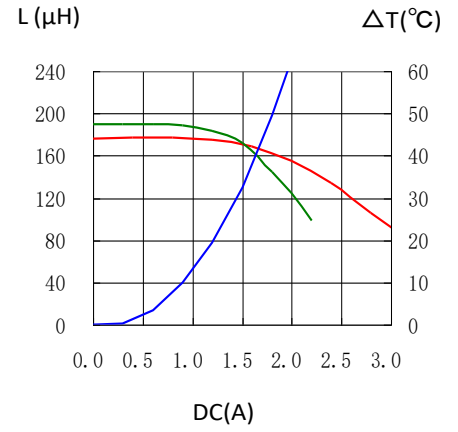
CDRH127/HPNP-181MC
