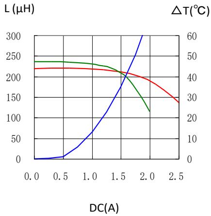
CDRH127/HPNP-221MC
