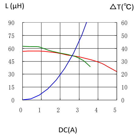
CDRH127/HPNP-560MC
