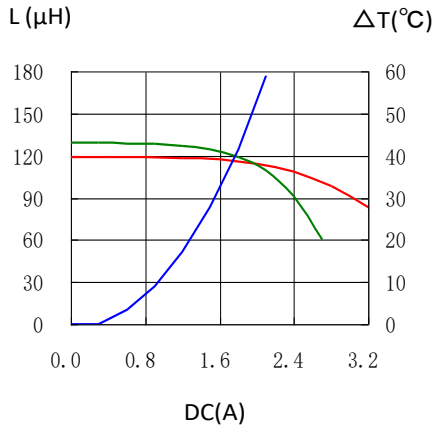
CDRH127/HPNP-121MC
