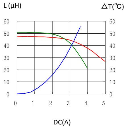
CDRH127/HPNP-470MC
