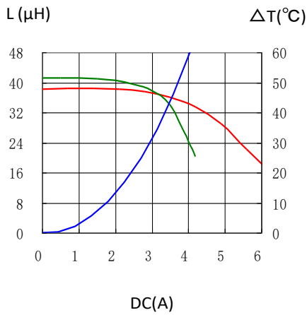
CDRH127/HPNP-390MC
