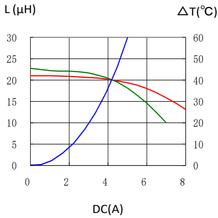
CDRH127/HPNP-220MC
