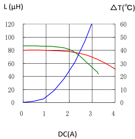
CDRH127/HPNP-820MC
