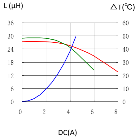
CDRH127/HPNP-270MC
