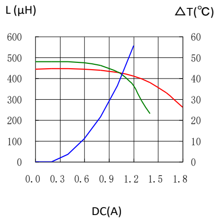
CDRH127/HPNP-471MC
