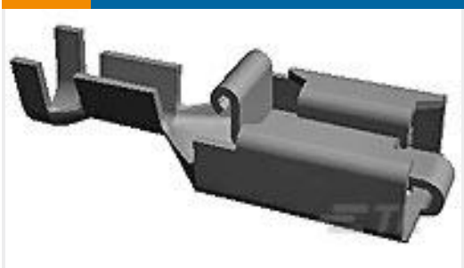
TE Part #927882-8 POS LOCK RECEPTACLE 6,3
