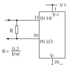
Links 1, 2, 3, 4 SHORTED.
