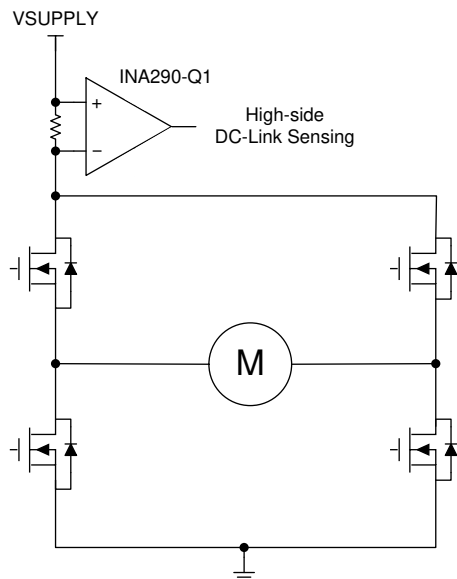
Figure 8-2. Current Sensing in a Automotive Pump
