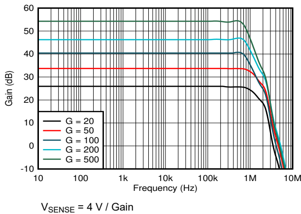
Figure 6-9. Gain vs Frequency
