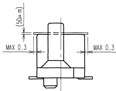
DETAIL FOR TAPE FOR VACUUM PICK-UP ( 5 : 1 )
