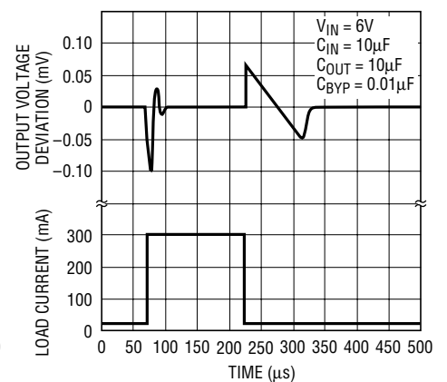
LT1962-5 Transient Response
