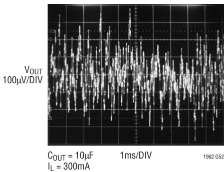
LT1962-5 10Hz to 100kHz Output Noise ( C_{BYP} = 0 )
