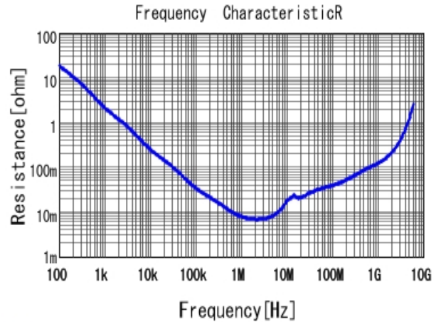
■ GRM188R61E225KA12 R DC0V, 25degC
