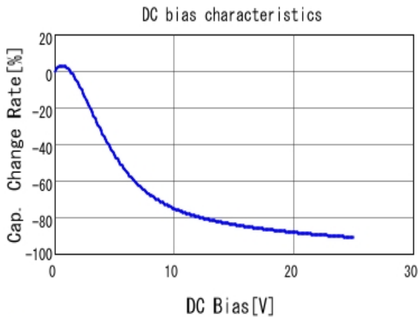
■ GRM188R61E225KA12 C-DC bias capchange, 25.0degC, AC1.
