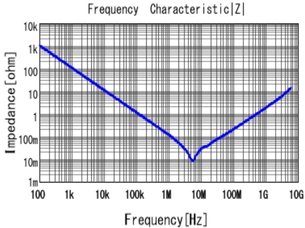
■ GRM188R61E225KA12 |Z| DC0V, 25degC
