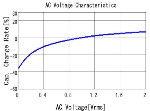
■ GRM188R61E225KA12 C-AC Voltage capchange, DC0V, 25.0d
