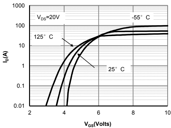
Figure 3: Transfer Characteristics
