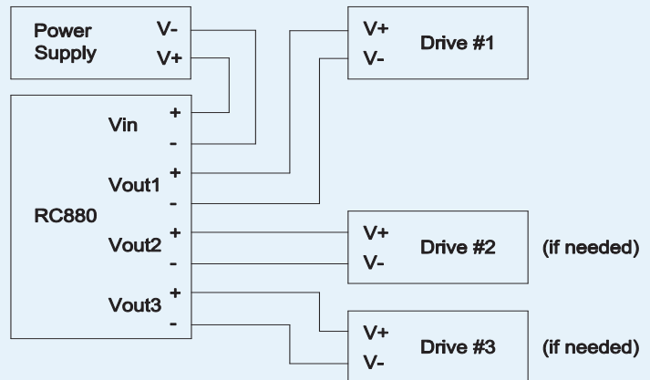
WIRING DIAGRAM
