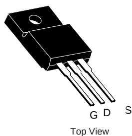
TO-220 FULLPAK
