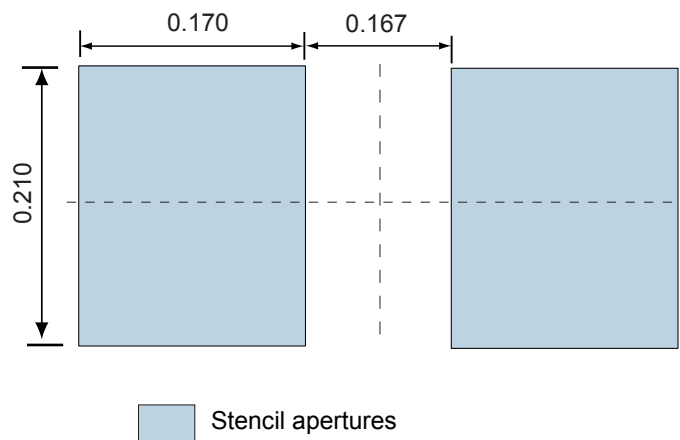
Figure 12. Stencil opening recommendations
