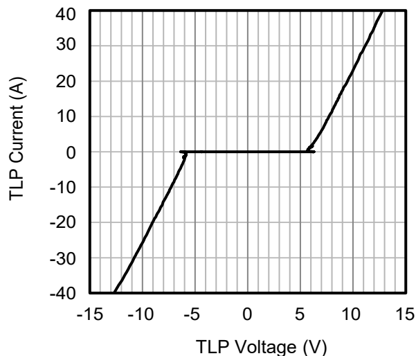
Fig4. TLP Measurement
