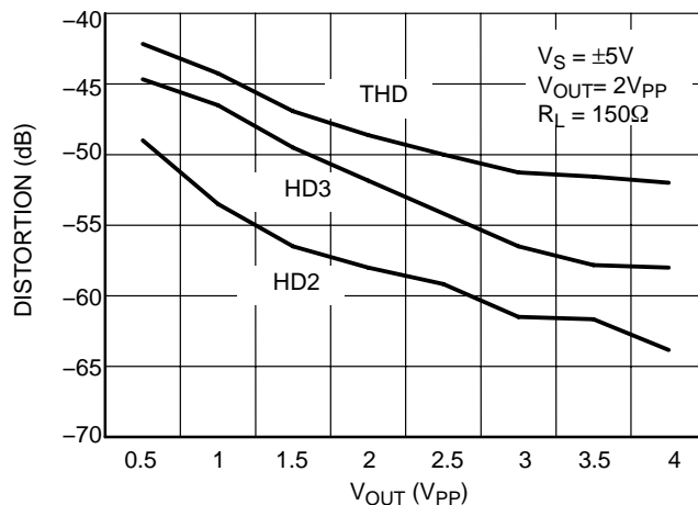
Figure 12. THD and Harmonic Distortion (dB) vs Output Voltage (V PP )
