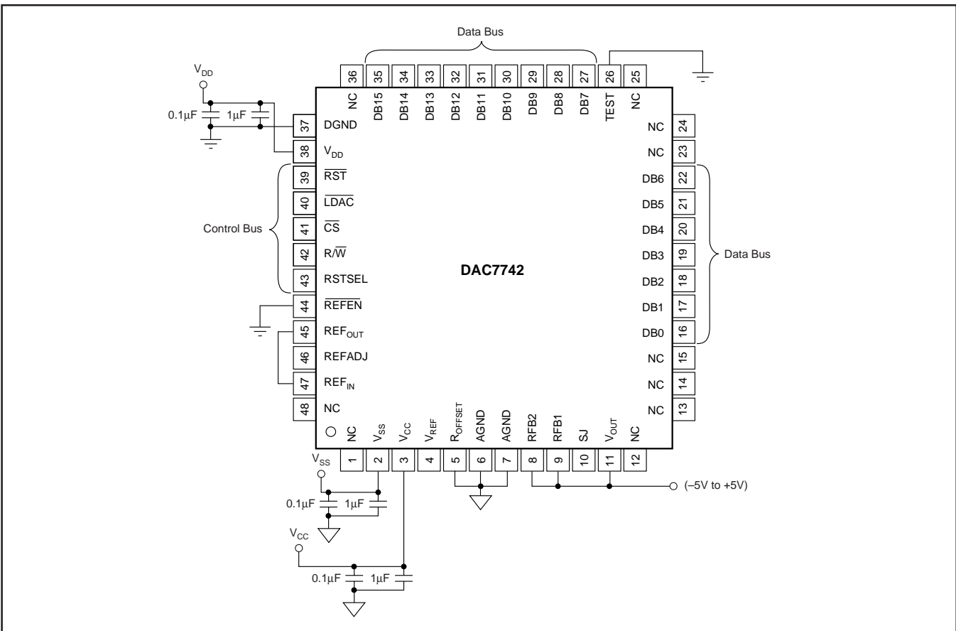
FIGURE 3. Basic Operation: V_{OUT} = -5V \text{ to } +5V .
