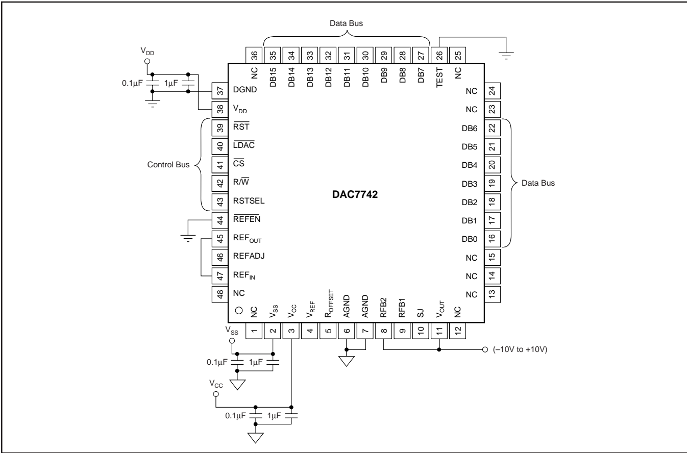
FIGURE 4. Basic Operation: V_{OUT} = -10V \text{ to } +10V .
