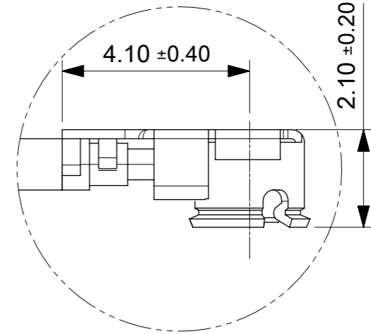
DETAIL A SCALE 17:2 CONNECTOR
