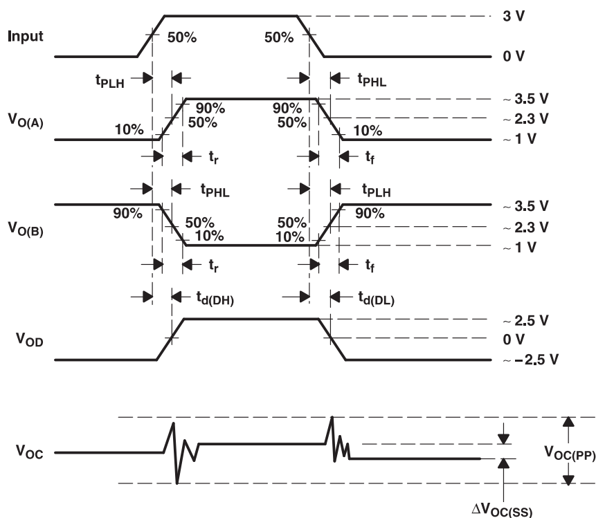
Figure 9. Driver Timing, Voltage, and Current Waveforms
