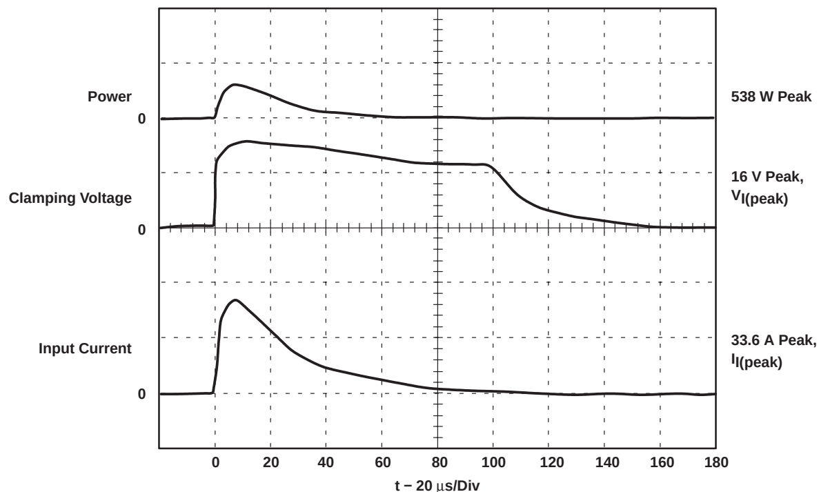
Figure 16. Typical Surge Waveform Measured At Terminals 5 and 7
