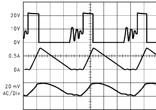
Discontinuous Mode Switching Waveforms
