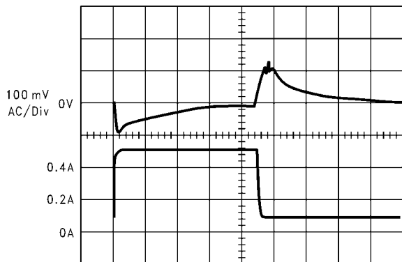
Load Transient Response for Continuous Mode
