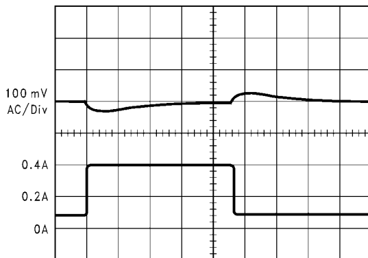
Load Transient Response for Discontinuous Mode
