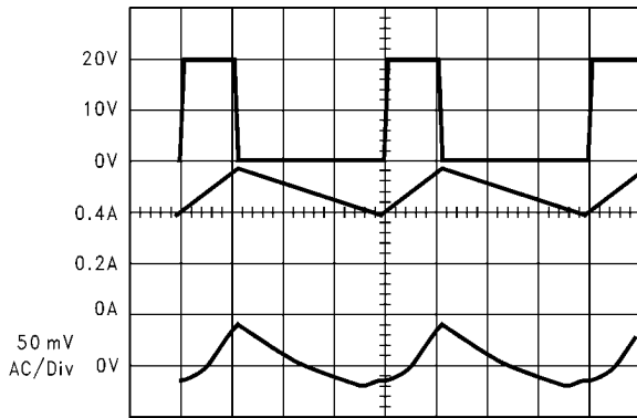
Continuous Mode Switching Waveforms
