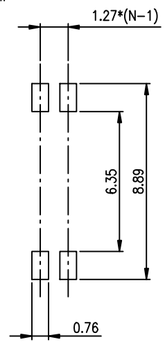
RECOMMENDED P.C.B. LAYOUT (TOP VIEW)
