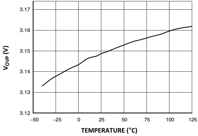
Figure 17. V OVP vs. Junction Temperature
