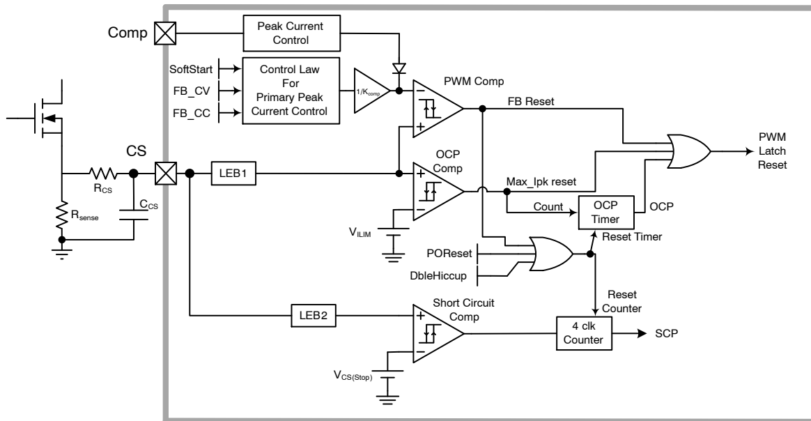
Figure 37. Current Setpoint
