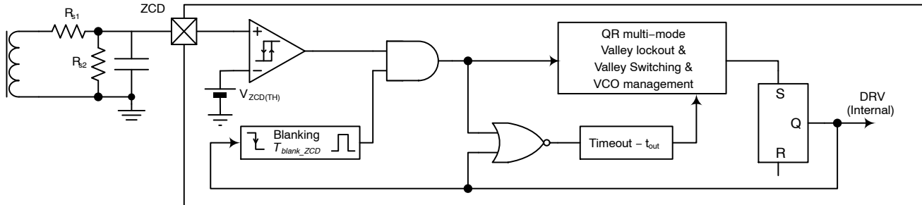
Figure 33. Valley Lockout Detection Circuitry Internal Schematic
