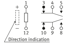
Schematic ( BOTTOM VIEW ) ( De-energize )
