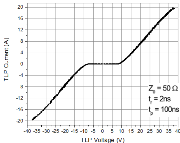
Fig3. TLP Measurement
