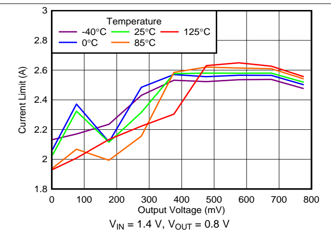
Figure 12. Current Limit Foldback
