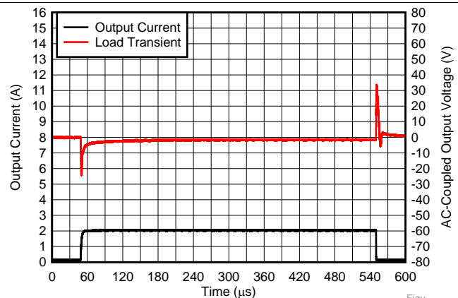
Figure 30. Load Transient Response ( V_{OUT} = 5.0\text{ V} ) V_{IN} = 5.5\text{ V} , I_{OUT} = 100\text{ mA to } 2\text{ A to } 100\text{ mA at } 1\text{ A}/\mu\text{s} , C_{OUT} = 22\text{ }\mu\text{F} , V_{PG} = V_{OUT}
