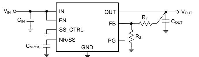
Figure 38. Adjustable Operation
