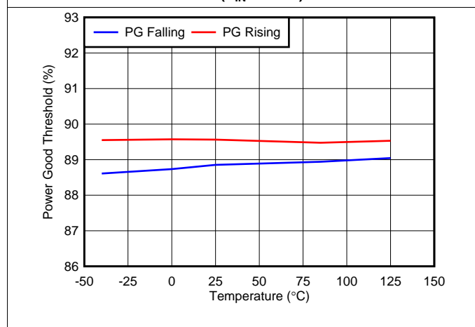
Figure 23. PG Threshold vs Temperature
