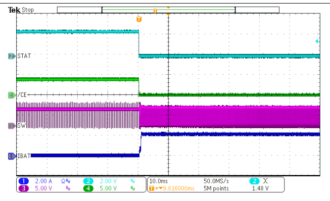
Figure 37. Charge Enable
