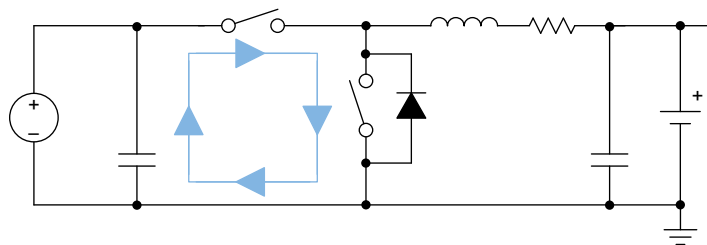
Figure 50. High Frequency Current Path
