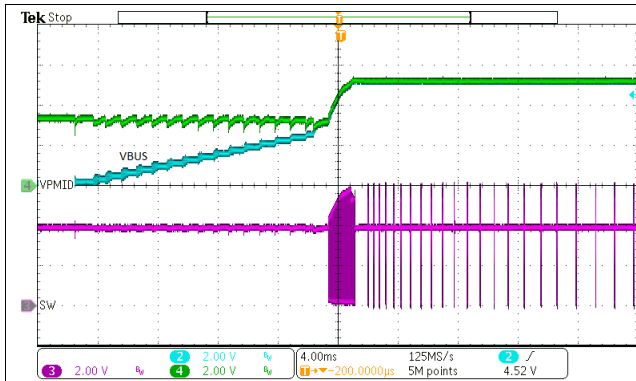
Figure 48. OTG Start-Up
