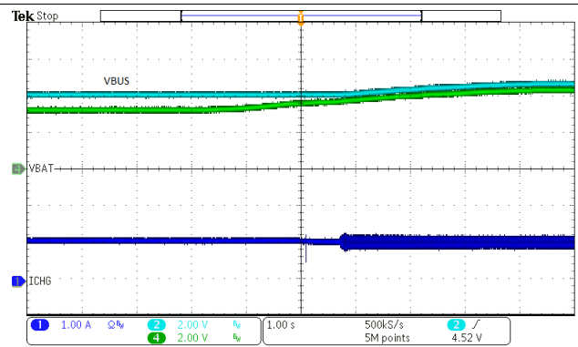
Figure 49. VINDPM Tracking Battery Voltage
