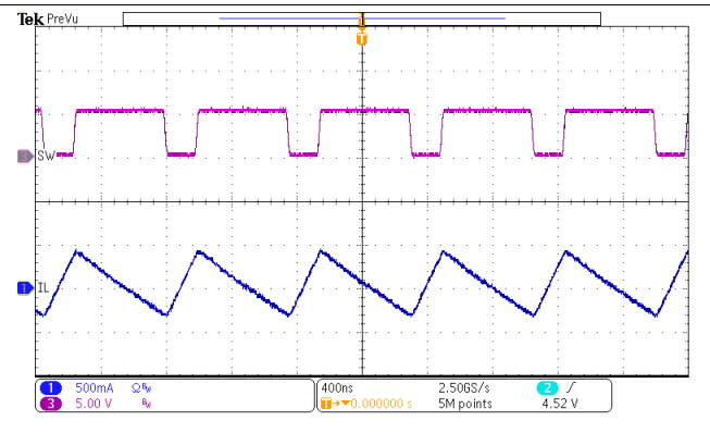
Figure 39. OTG Switching
