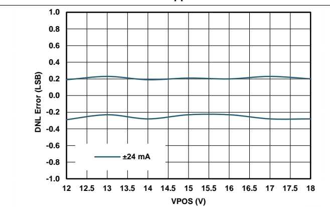
Figure 16. IOU T Differential Linearity Error vs Power Supplies
