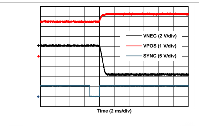
Figure 84. Buck-Boost Converter Power-On (VOUT Mode)
