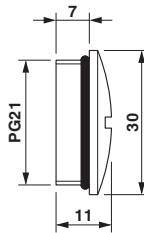
Dimensional drawing
