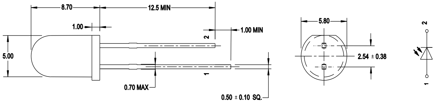
Figure 1: Package Drawing
