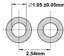
Figure 9: Recommended PCB Through-Hole Size
