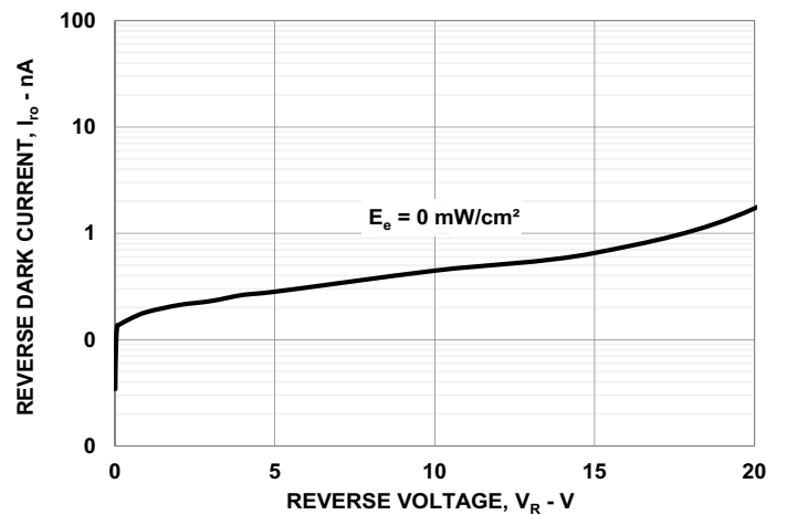
Figure 5: Reverse Dark Current vs. Reverse Voltage
