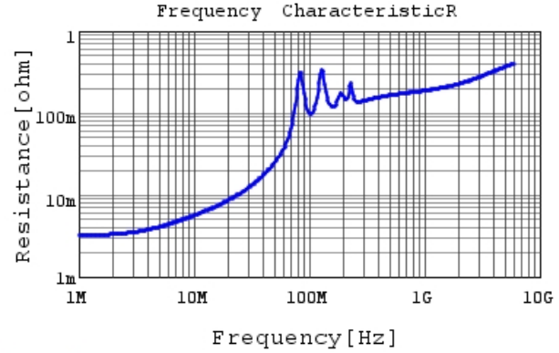
GRM21B5C1H223JA01 R DCOV, 25degC
