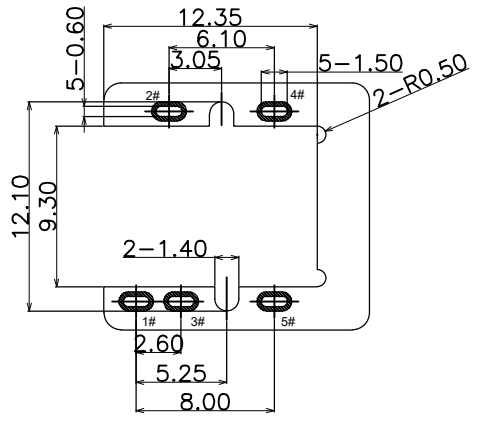
PCB LAYOUT (TOP VIEW) TOLERANCE: ±0.05
