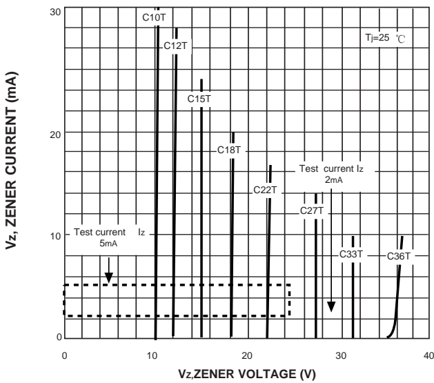
FIG. 3-ZENER BREAKDOWN CHARACTERISTICS
