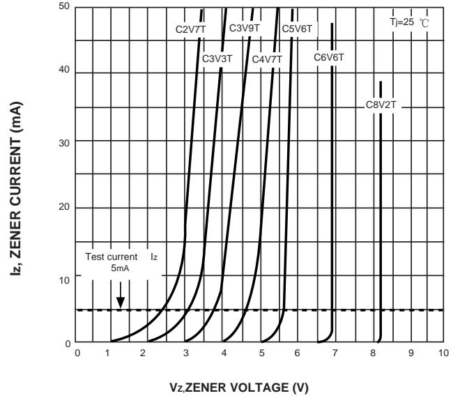
FIG. 2-ZENER BREAKDOWN CHARACTERISTICS
