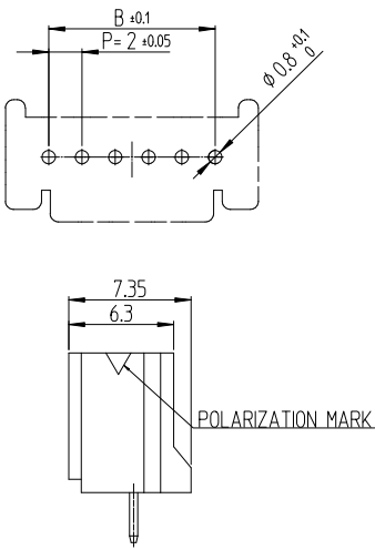
Recommended PCB Layout (t=1.6mm)
