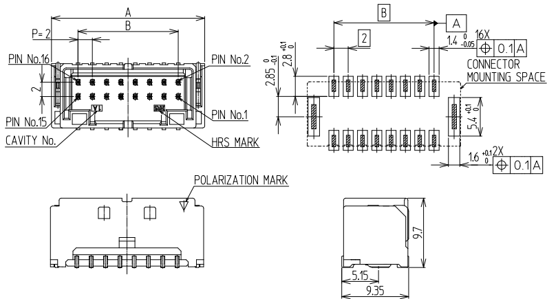
Recommended PCB Layout (t=1.6mm)
