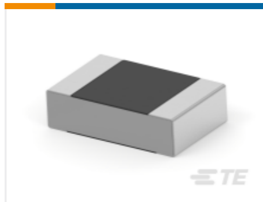
TE Part #5-2176264-9 RN 0805 4R75 0.1% 10PPM 1K RL
