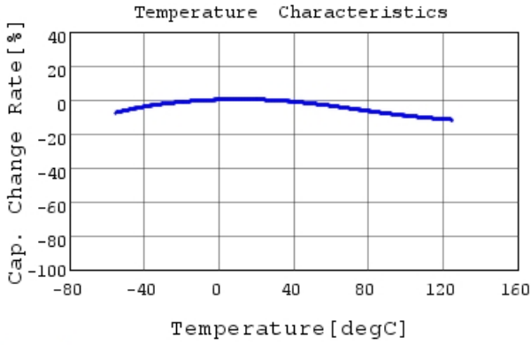
GRM21BR71A225KA01 C-Temp. capchange, DC0.0V,
