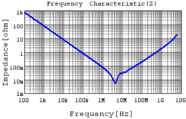
GRM21BR71A225KA01 |Z| DCOV, 25degC
