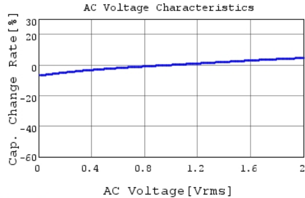
GRM21BR71A225KA01 C-AC Voltage capchange, Dc
