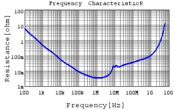
GRM21BR71A225KA01 R DCOV, 25degC
