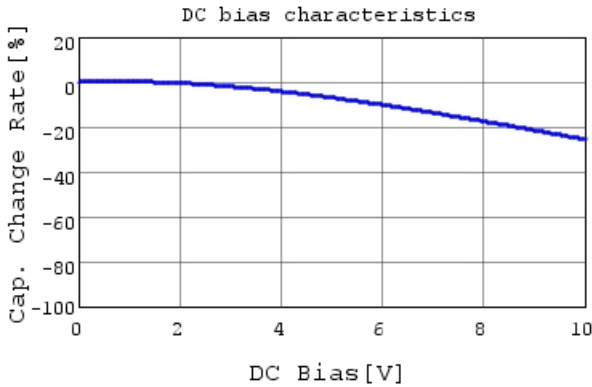
GRM21BR71A225KA01 C-DC bias capchange, 25.0c
