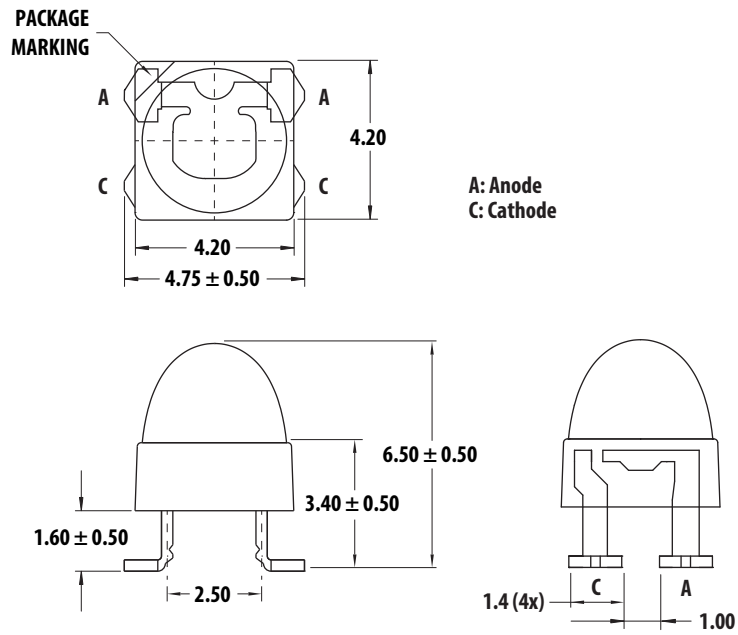
Figure 1 Package Dimensions
